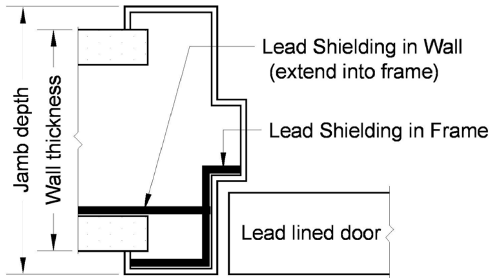
TYPE 1 FRAME
