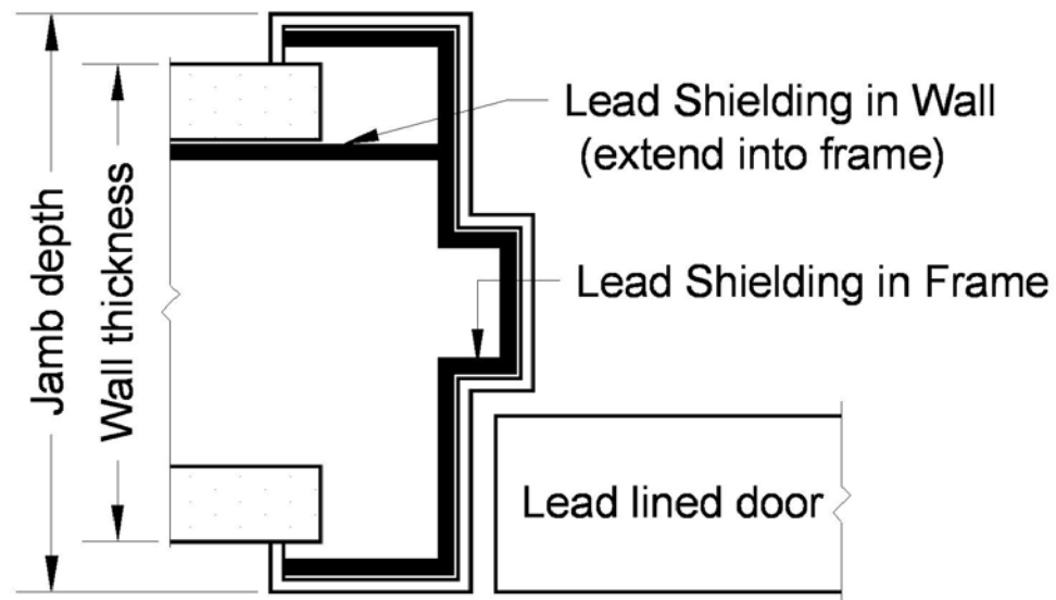
TYPE 2 FRAME
